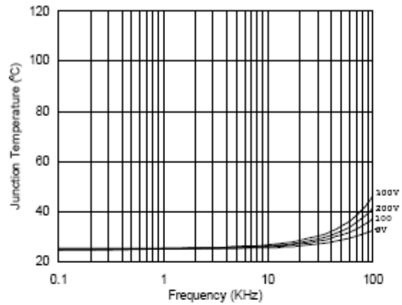
Figure 50. IR2136/IR21362(3)(5)(6)(7)(8) (S) vs. Frequency (IRG4BC30W), R gate =15Ω, V cc =15V
